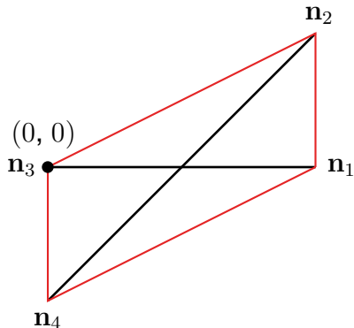
Figure 2.3: Planar tensegrity cross subject to affine node transformation
