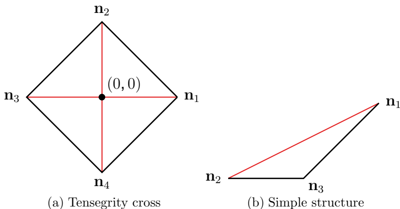
Figure 2.4: Dual structures
