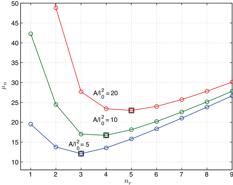
Figure 3.42: Three-bar tensegrity plate: \mu_n versus n_r , for \epsilon = 0.05 and A/\ell_0^2 = \{5, 10, 20\} , from (3.62) using (3.64) and (3.65)
