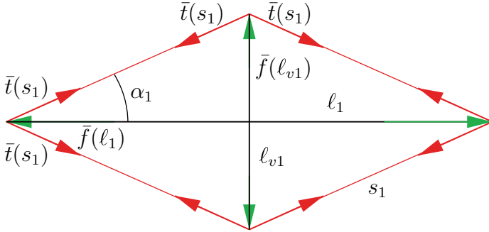
Figure 3.5: T-Bar forces for unloaded (prestressed) case, f(\ell_0) = 0
