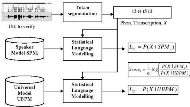
Fig. 8.3. Verification of an utterance against a speaker model in phonotactic speaker recognition
