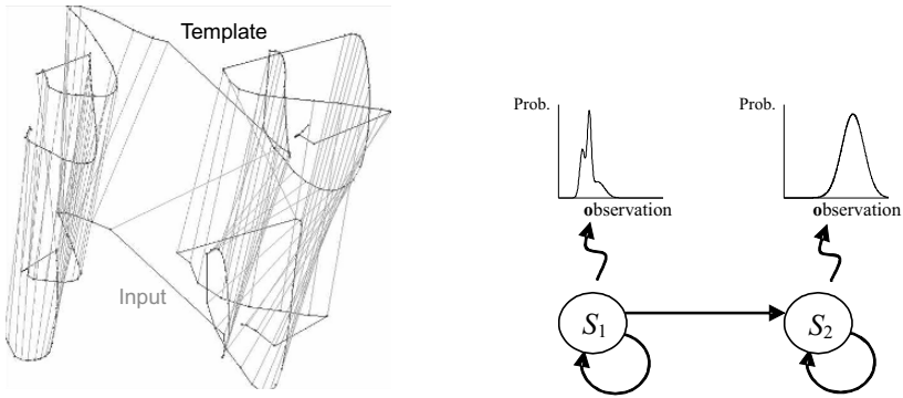
Fig. 10.3. Example of local elastic matching of signatures based on DTW (left, Chinese signature from SVC 2004) and regional modeling based on HMM (right).
