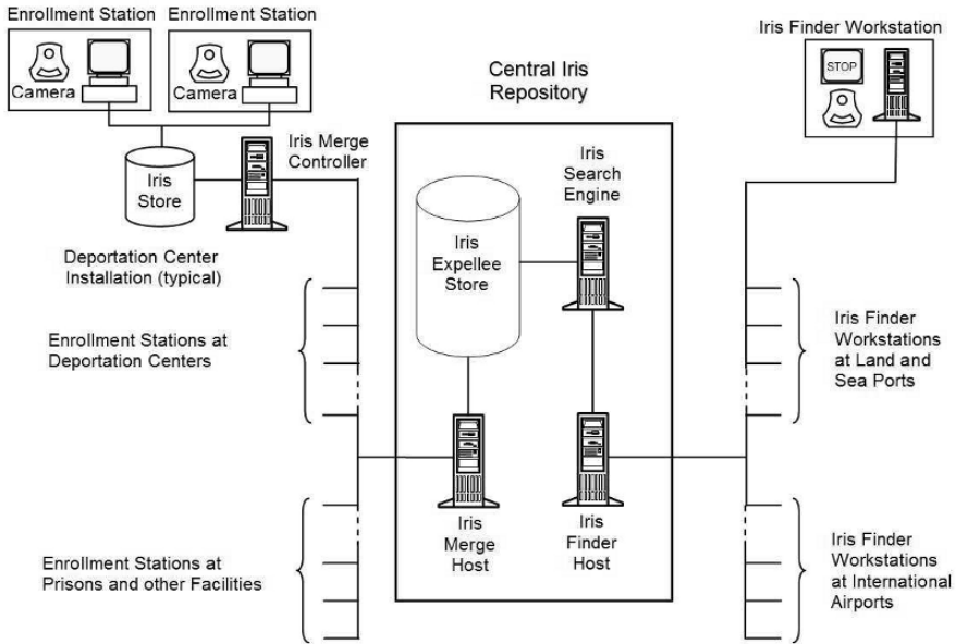
Fig. 22.1. System Architecture.
