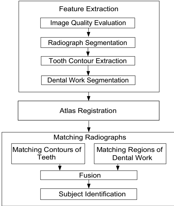
Fig. 12.4. Block diagram of automatic dental identification system.
