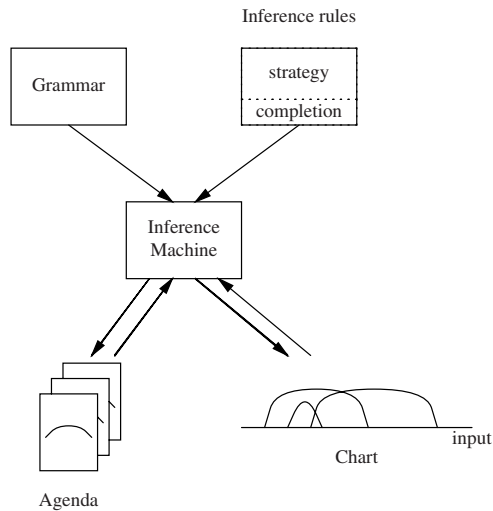
Fig. 7.27. The agenda in chart parsing
