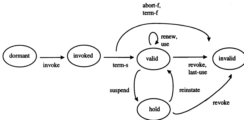
Figure 5. Basic processing states for an authorization-step
