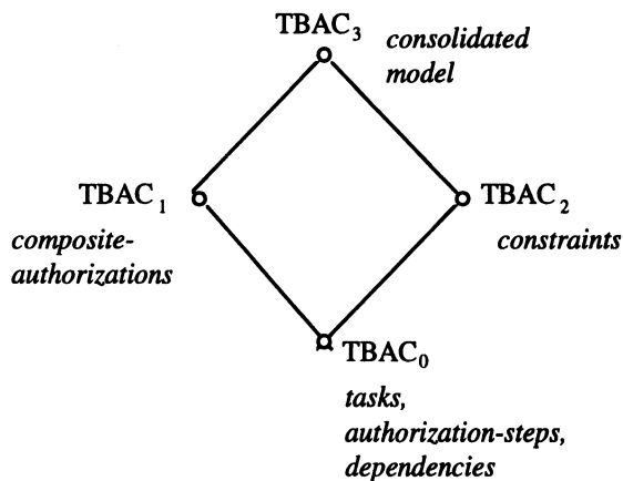
Figure 4. A framework for a hierarchy of TBAC models
