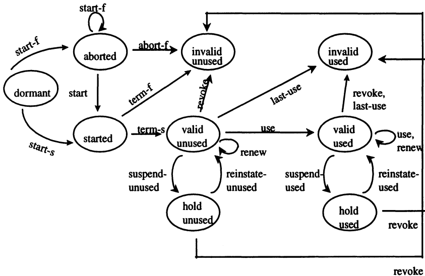
Figure 6. Detailed processing states of an authorization-step
