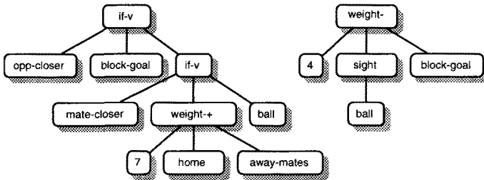
Fig. 3. The subtree crossover operator in action. This operator swaps subtrees among two genomes.
