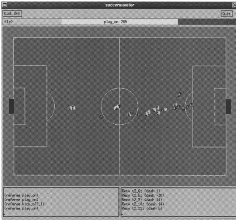
Fig. 7. Some players begin to hang back and protect the goal, while others chase after the ball.
