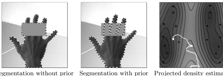
Fig. 7. Segmentation with a nonlinear shape prior containing right (+) and left (•) hands — shown in the projected energy plot on the right. The input image is a right hand with an occlusion. After the Mumford–Shah segmentation becomes stationary (left image), the nonlinear shape prior is introduced, and the contour converges towards the final segmentation (center image). The contour evolution in its projection is visualized by the white curve in the energy density plot (right). Note that the final segmentation (white box) does not correspond to any of the training silhouettes, nor to the minimum (i.e. the most probable shape) of the respective cluster.
