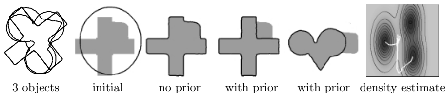
Fig. 6. Segmentation of artificial objects (left) with nonlinear shape prior: the same prior can encode very different shapes. Introduction of the shape prior upon stationarity of the contour causes the contour to evolve normal to the level lines of constant energy into the nearest local minimum, as indicated by the white curves in the projected density estimate (right).
