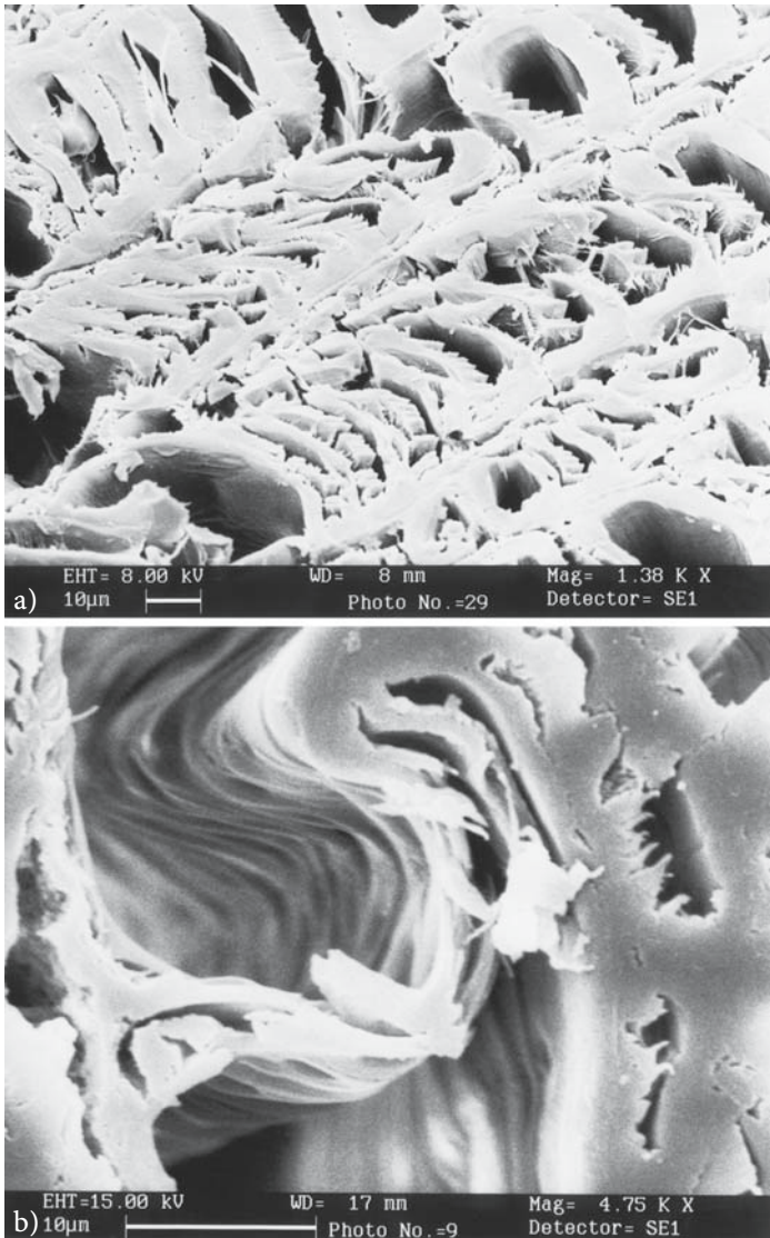
Fig. 6.9. Micrographs of spruce and cherry following compaction under hydrostatic pressure (Bucur et al. 2000). a Spruce in the RT plane. The shear effect can be seen by the corrugation of cell walls. b Cherry in the RT plane. Corrugation of the wall of a vessel: the quasi-circular section of vessels becomes irregularly elliptical as a result of shear deformation of the structure. The fibers around the deformed vessel also appear very much compressed. Only fibers of relatively small diameter maintained the original transversal section shape
