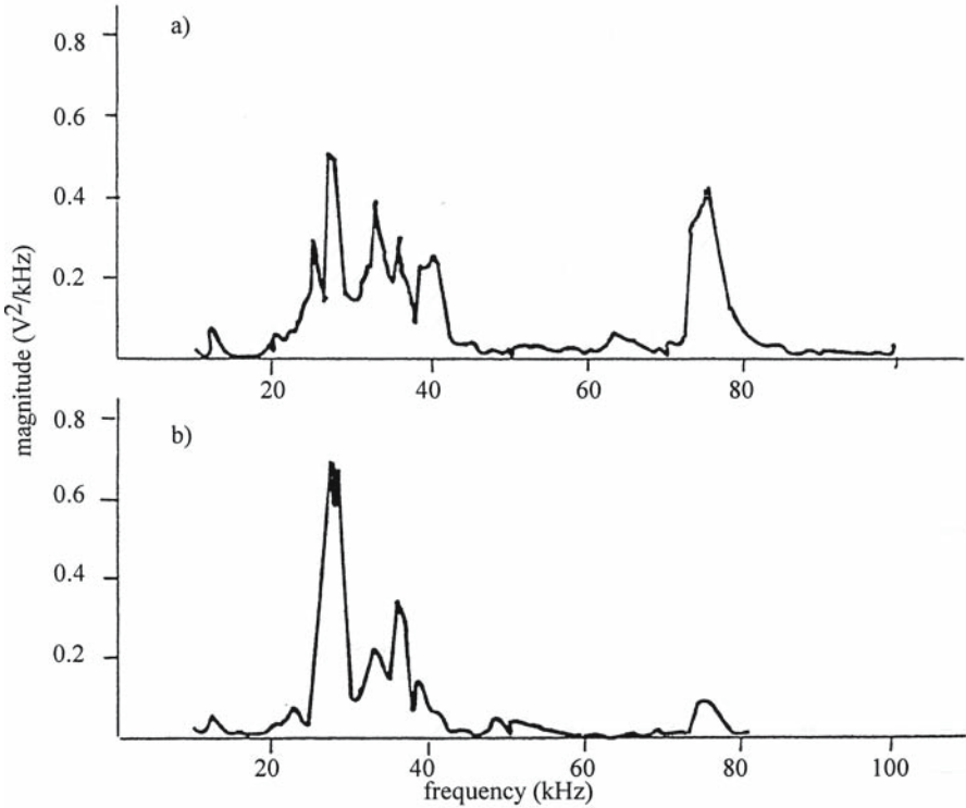
Fig. 9.13. Frequency spectra of received wave from a specimen attacked by fungi and from a sound specimen. a Control specimen; b specimen exposed to fungi for 5 days. (Patton-Mallory and DeGroot 1989, with permission)
