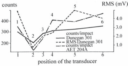
Fig. 10.32. Acoustic emission parameters (counts, RMS voltage) during scanning of a ponderosa pine board with an encased knot of 6 cm. (Lemaster and Dornfeld 1987, with permission)
