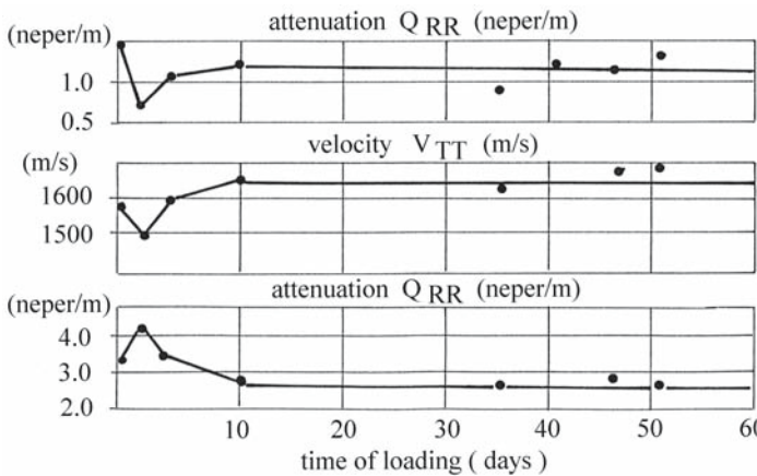
Fig. 7.20. Spruce. Radial static bending loading at 0.2 \sigma_{rupture} . Relationship between ultrasonic velocity, attenuation, and time of loading. (Bucur 1980a)
