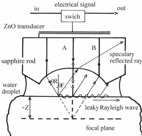
Fig. 5.10. Signal reflected by the specimen as a result of interference between the surface Rayleigh wave (B) and longitudinal wave reflected at normal incidence (A). (Atal 1989)
