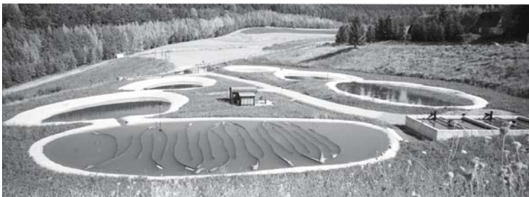
Fig. 7. Photograph of the constructed wetland at Poehla, Autumn 2004.
