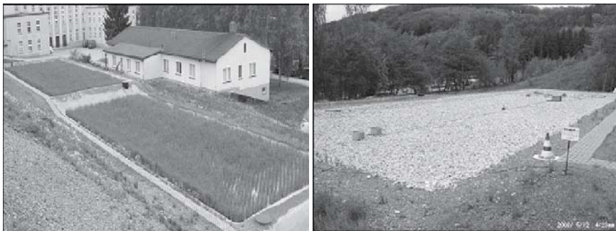
Fig. 8. Experimental multi-cell wetland at WISMUT's Schlema mine site (left: plant cells, right: microbiological cell with gravel bed).
