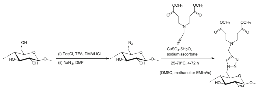
Fig. 31 Reaction path for conversion of cellulose with first generation propargyl-PAMAM dendron via tosylation, nucleophilic displacement by azide, and conversion with the dendron
