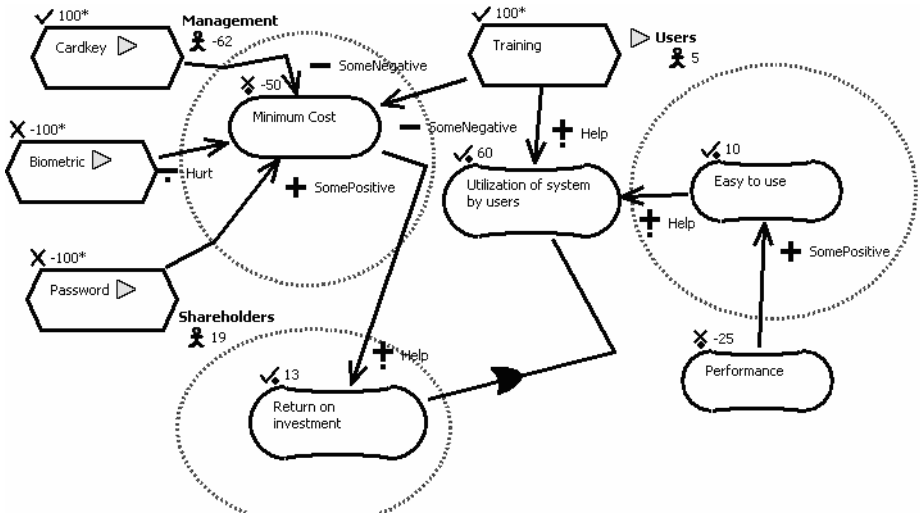
Fig. 12. GRL diagram annotated with links and actor evaluations
