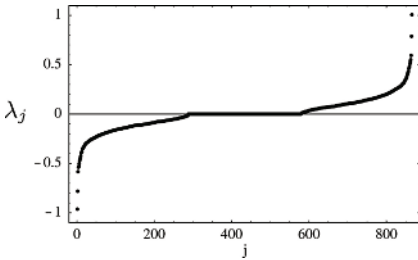
Fig. 7. Eigenspectrum of the SUMO ontology sorted by value
