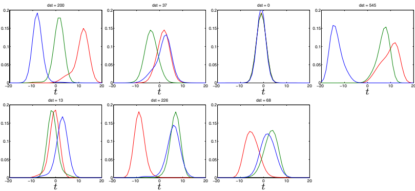
Fig. 6. Histogram cross-correlation (h_3^{c_{\{1,2,3\}}} \star h_j^{c_{\{1,2,3\}}})(t) for j = 1..7 . Red, green, blue colour of the curves in each graph corresponds to the c_1, c_2, c_3 colour channel respectively.
