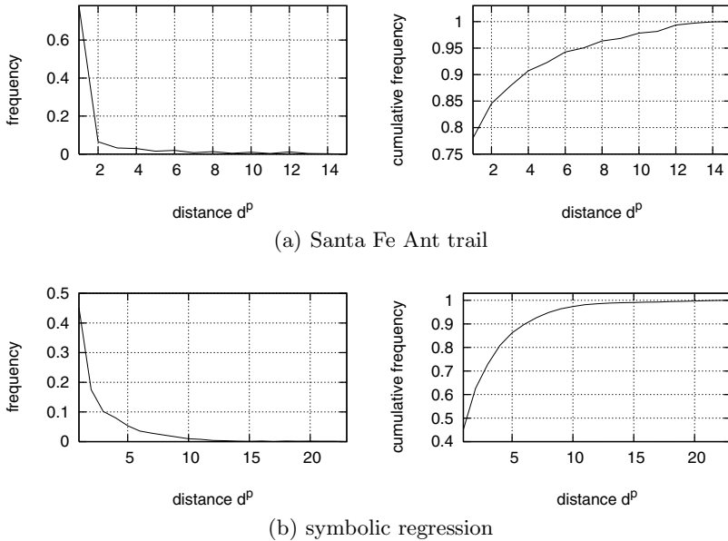
Fig. 2. Distribution of tree edit distances d^p_{x,y} for neighboring genotypes x and y , where d^g_{x,y} = 1 . We show the frequency (left) and cumulative frequency (right) over d^p_{x,y} for the Santa Fe Ant trail problem and the symbolic regression problem.
