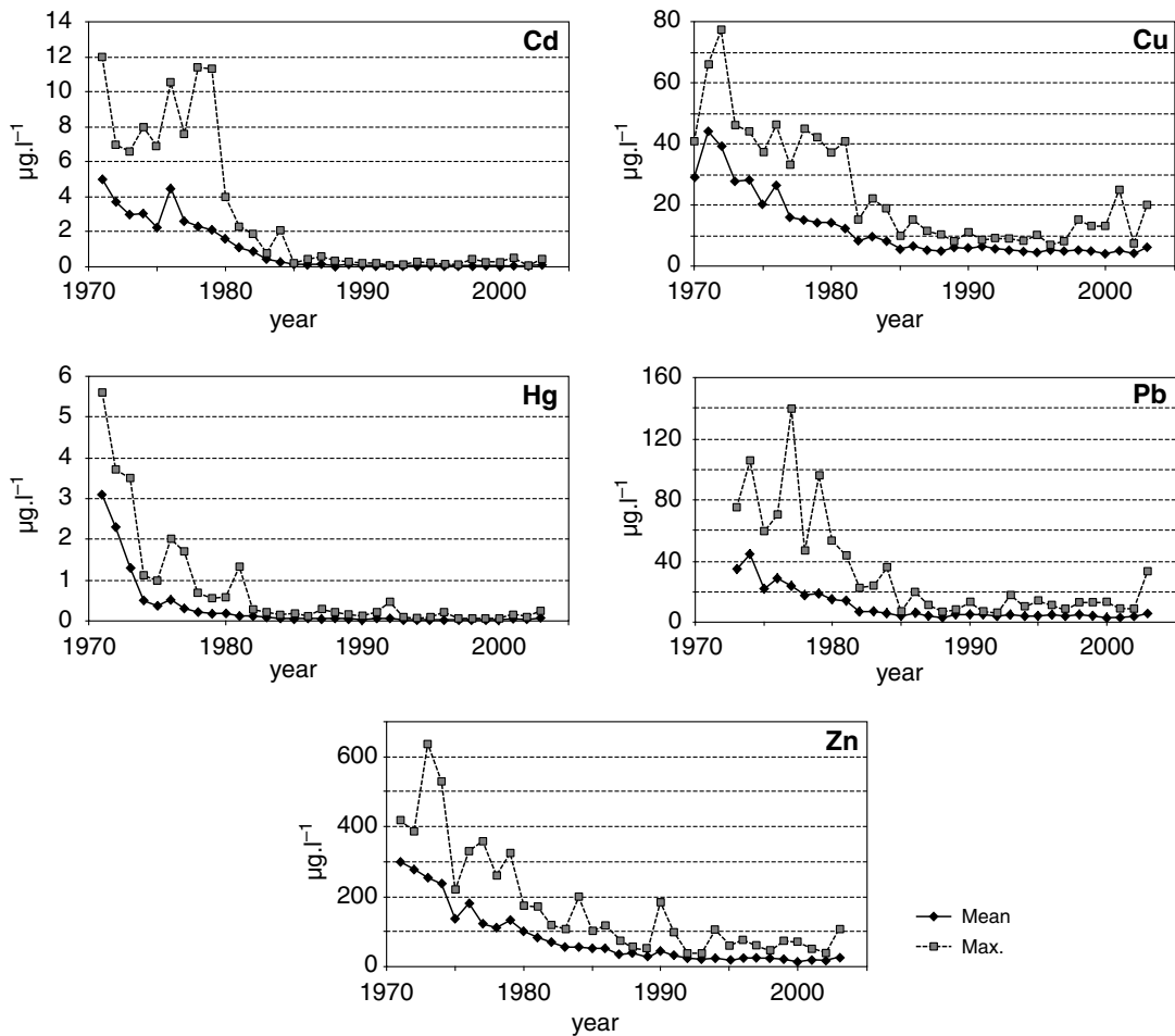
Figure 4. Yearly average and maximum observed total concentrations of Cd, Cu, Hg, Pb and Zn in the river Rhine measured at the German–Dutch border.
