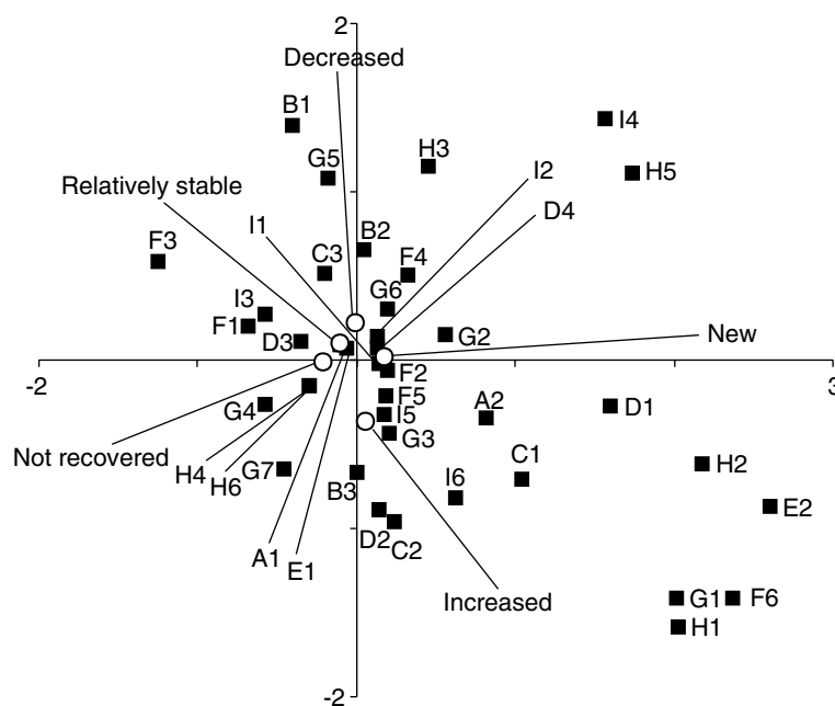
Figure 5. Plot of the first two axes of the correspondence analysis of biological traits. Squares and codes represent classes of biological traits (Table 2): flight capability (A), preferred life history (B), diet of juveniles (C), diet of adults (D), reproduction (E), parental care (F), respiration of juveniles (G), respiration of adults (H) and preferred habitat (I). Changes in the density of species are plotted as open circles: species found only before restoration (“Not recovered”), species with a density decrease of more than 25% (“Decreased”), species with a density change of less than 25% (“Relatively stable”), species with a density increase of more than 25% (“Increased”) and species found only after restoration (“New”).
