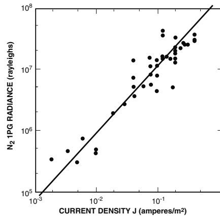
Figure 8. The measured radiance of the positive column of the large glow discharge tube versus the current density, computed as the total current divided by the cross-sectional area of the tube.
