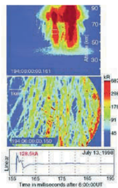
Figure 11. Telescopic imagery on an angel sprite (Gerken et al., 2000), showing detailed filamentary structure.
