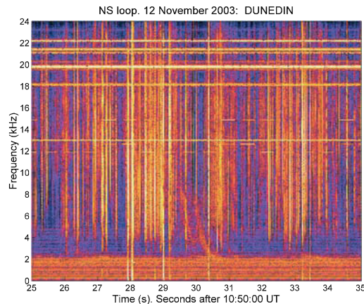
Figure 1. A VLF/ELF spectrum showing data received by a north-south aligned magnetic loop antenna located near Dunedin, New Zealand during the local nighttime. Strong VLF transmitters and lightning signals are present, with the strongest man-made transmitter being NWC at 19.8 kHz. A weak and “swishy” whistler is also present at \sim 30 s.
