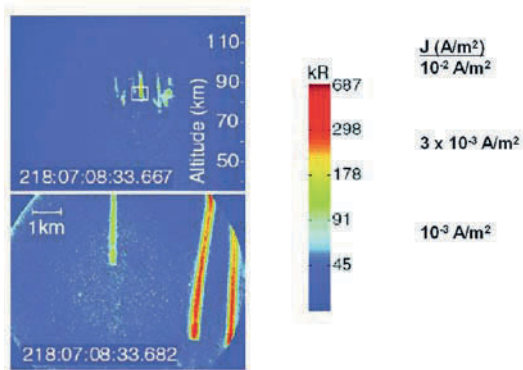
Figure 10. Telescopic imagery on column sprites (Gerken et al., 2000), showing isolated luminous channels. The scale for current density is based on results in Figure 8.
