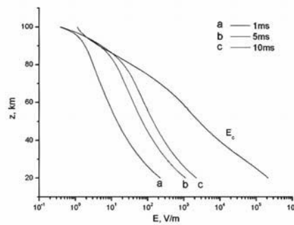
Figure 4. Electric field profiles during the continuous current stage at selected instants for the current I = 10 kA.
