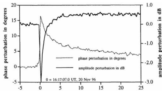
Figure 5. Relaxation of a large VLF perturbation observed on transmissions from NWC at Darwin, Australia. This is believed to be a VLF sprite perturbation. The x-axis in seconds after the origin time (reproduced with permission of American Geophysical Union ©1997; Dowden et al., 1997).
