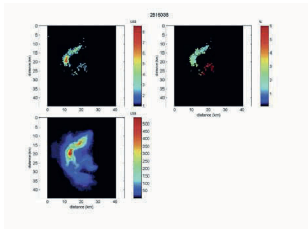
Figure 6. Simultaneous observation of a sprite and a superbolt performed on October 3 rd , 2003, at 19:19:31 UT at 35.58°N 36.18°E. The ratio of both cameras is higher than 6 for the sprite. It is about 1% for the superbolt. The most intense event in the visible and in the filter corresponds to a ratio of 2 to 3% and could be explained by the presence of a halo.
