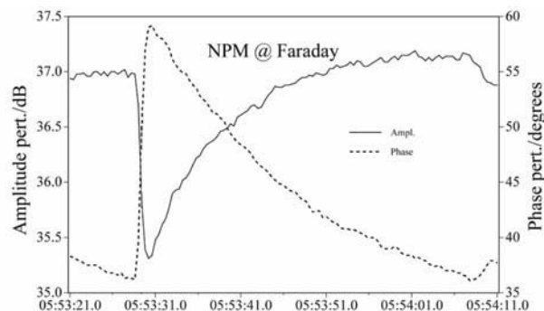
Figure 3. Example of a classic Trimp perturbation observed on transmissions from the US Navy transmitter NPM (Hawaii; then 23.4 kHz) at Faraday (Antarctic Peninsula) on 23 April 1994. In this case the amplitude (solid line) decreases, while the phase (dotted line) increases (reproduced by permission of American Geophysical Union ©2001; Dowden et al., 2001b).
