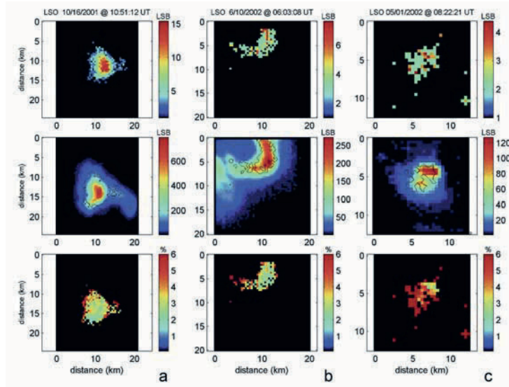
Figure 5. First observation of sprite from the nadir by LSO. 1. Top filtered images 2. Middle: images in the visible, 3. Bottom: ratio of both intensities. The event at the right is a superbolt while both events on the left are sprites. They are differentiated by the ratio of the intensities measured by both cameras, most intense for sprites than for lightning.
