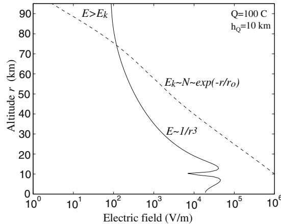
Figure 2. Physical mechanism of sprites Wilson (1925): “While the electric force due to the thundercloud falls off rapidly as r increase, the electric force required to causing sparking (which for a given composition of the air is proportional to its density) falls off still more rapidly. Thus, if the electric moment of a cloud is not too small, there will be a height above which the electric force due to the cloud exceeds the sparking limit.”
