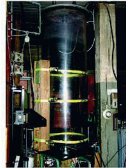
Figure 2. Photograph of the large discharge tube used in the present study.
