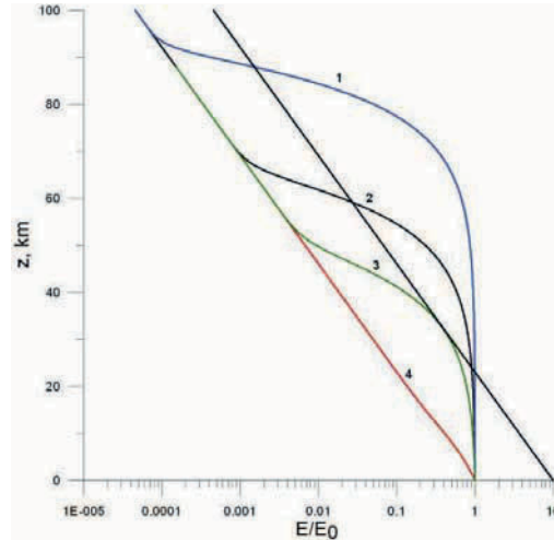
Figure 1. Transition process after instant switching of the electric field at the boundary, 1: t/t_r = 0.001 , 2: t/t_r = 0.01 , 3: t/t_r = 0.04 , 4: t/t_r = 1 .
