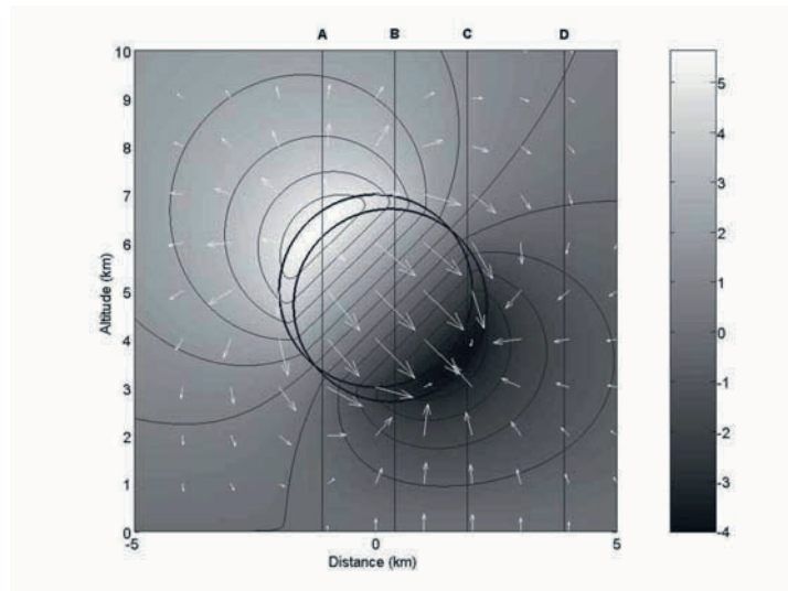
Figure 2. Spatial electric field structure in an atmospheric convective cell with cylindrical geometry and with the conducting Earth taken into account. Shades of gray correspond to different values of electric potential.
