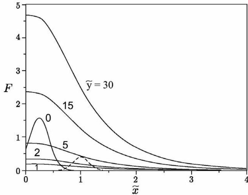
Figure 13. The velocity distribution function of electrons for the relativistic case; the different curves correspond to different values of the dimensionless variable \tilde{y}\phi_{\text{min}}t/p_0^3 .
