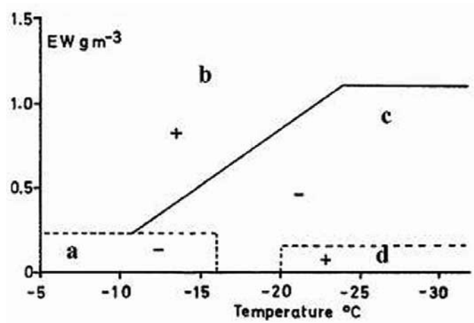
Figure 2. Charging regimes in the Effective Water Content (EW)-Temperature phase space, based on the results of laboratory experiments conducted by the UMIST group (Saunders et al., 1991, with permission).
