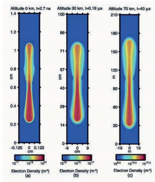
Figure 8. A cross-sectional view of the distribution of the electron number density of the model streamers at altitudes (a) 0 km, (b) 30 km, and (c) 70 km (Liu and Pasko, 2004). Reprinted by permission from American Geophysical Union.
