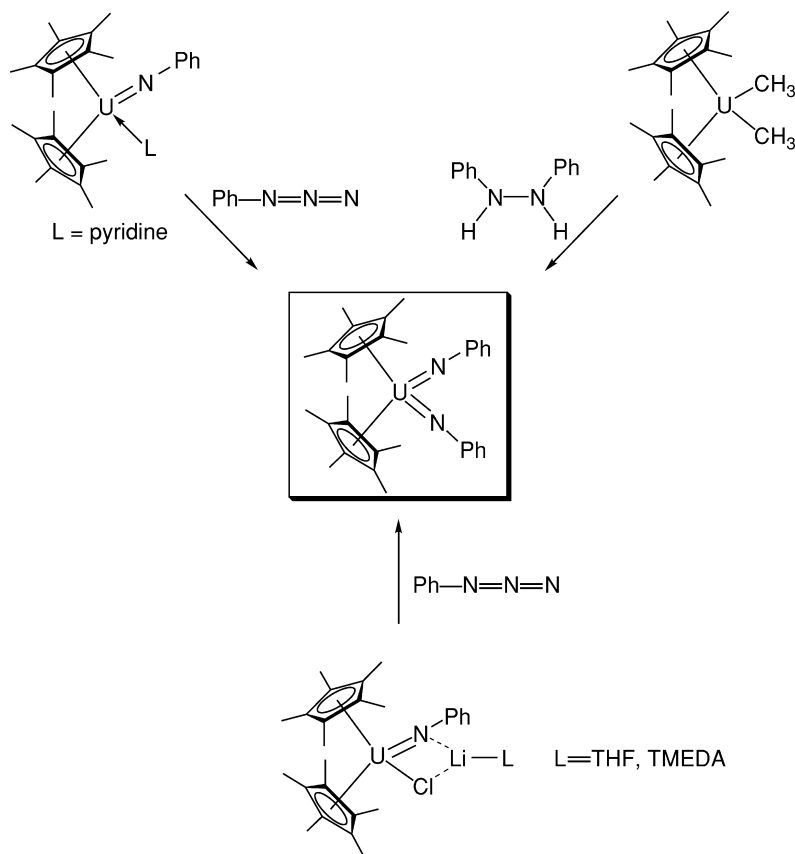
Fig. 25.19 Synthetic pathways to (\eta^5\text{-C}_5\text{Me}_5)_2\text{U(=NC}_6\text{H}_5)_2 (Arney et al. , 1995).
