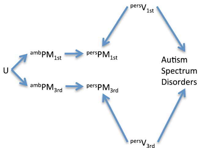
Fig. 3 Directed acyclic graph (DAG) representing the relations between ambient (amb superscripts) particulate matter (PM) concentration estimates, personal (pers superscripts) PM exposure estimates, time-invariant factors (U) that affect ambient PM, time-varying factors (V) that affect personal PM exposure, and autism spectrum disorders. The subscripts indicate different trimesters of pregnancy. The personal PM exposures are colliders. See text for additional discussion
