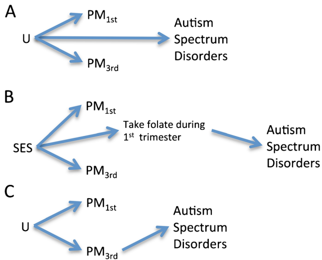
Fig. 1 Directed acyclic graphs (DAG) representing possible confounding of the particulate matter (PM)—autism spectrum disorders (ASD) association by time-invariant factors ( U ). The subscripts indicate different trimesters of pregnancy. Each panel depicts a different set of assumptions about the underlying factors that give rise to the data. a There is no causal effect of PM on ASD, but some U variables confound the PM–ASD association. b Same as a , with addition of folate consumption during 1st trimester of pregnancy as one way that SES (as one possible U variable) causes ASD. c Only PM_{3rd} is causally associated with ASD, while U and PM_{1st} are not. See text for additional discussion
