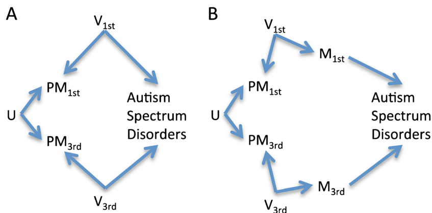
Fig. 2 Directed acyclic graphs (DAG) representing possible confounding of trimester-specific associations by time-varying factors. a Factors that vary from the 1st to 3rd trimester of pregnancy (V) could introduce confounding of the particulate matter (PM)—autism spectrum disorders (ASD) association that is specific to one of the trimesters. b
