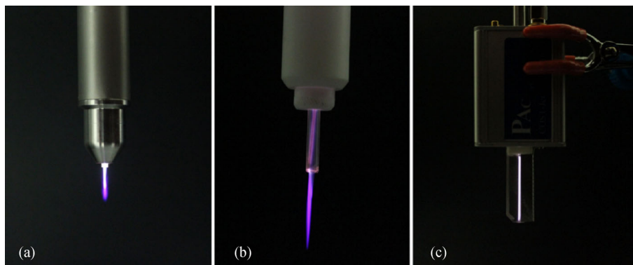
Fig. 1 Representative picture of three examples of plasma jets of interest in plasma medicine: (a) atmospheric pressure argon plasma jet (kINPen), (b) plasma needle, and (c) microplasma COST
