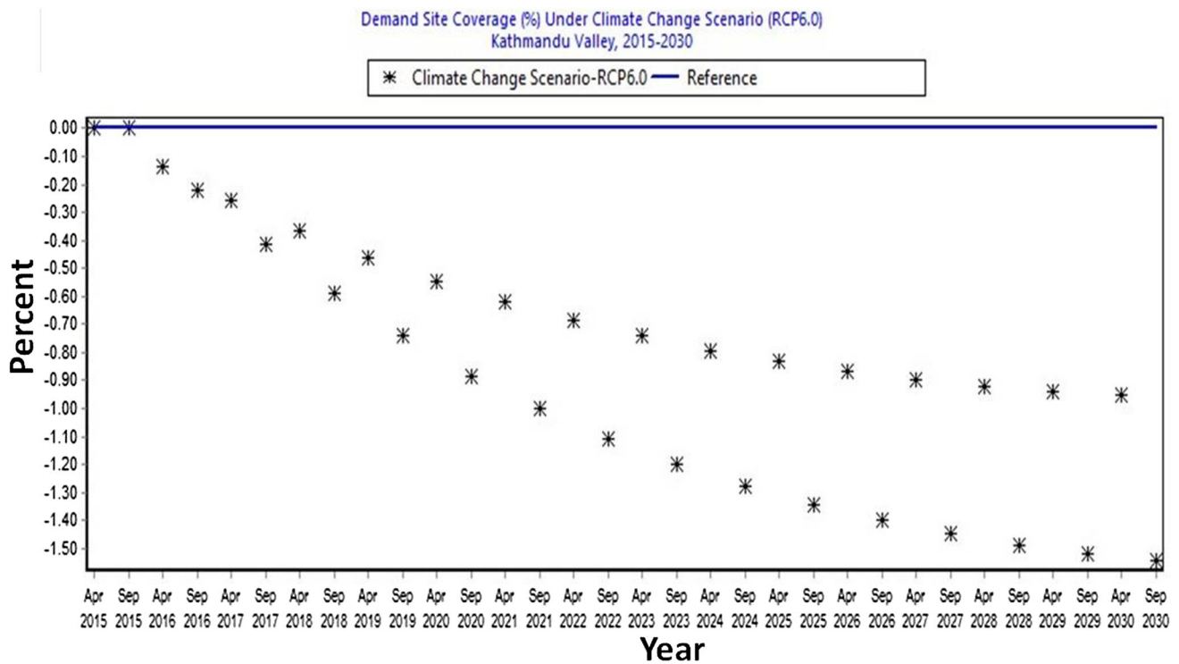
Fig. 9 Future projection of water demand coverage in Kathmandu Valley under climate change scenarios (2015–2030)
