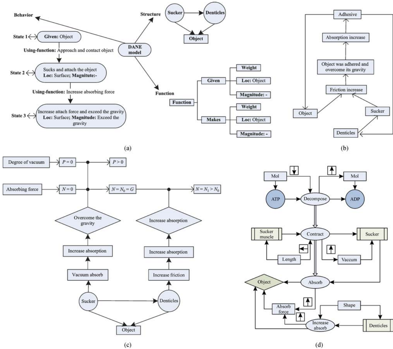
Fig. 3 Various diagrammatic models for the structure of octopus suckers. (a) DANE; (b) SAPPhIRE; (c) UNO-BID; (d) MBE. ATP is the abbreviation of adenosine triphosphate, ADP is the abbreviation of adenosine diphosphate, Mol is the physical unit for mole
