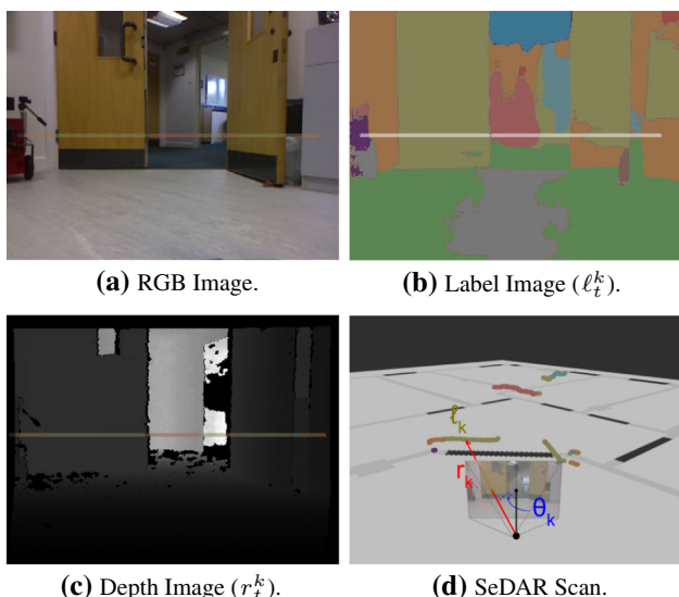
Fig. 4 Visualisation: sensor input, semantic segmentation and the resulting SeDAR scan
