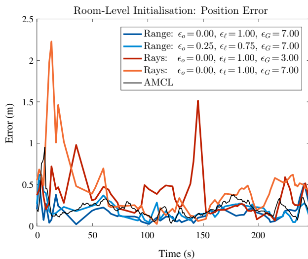
Fig. 7 Semantic floorplan localisation, room-level initialisation (Color figure online)
