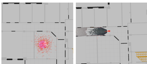
(a) Room-Level Initialisation (b) AMCL [10]
