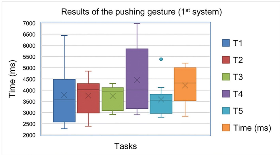
Fig. 21 Results Box plot of the pushing gesture (1st system)
