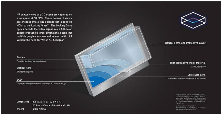
Fig. 13 The Looking Glass 15.6'' development kit
