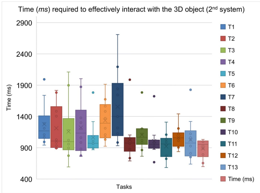
Fig. 23 Results box plot of interaction effectiveness (2nd system)
