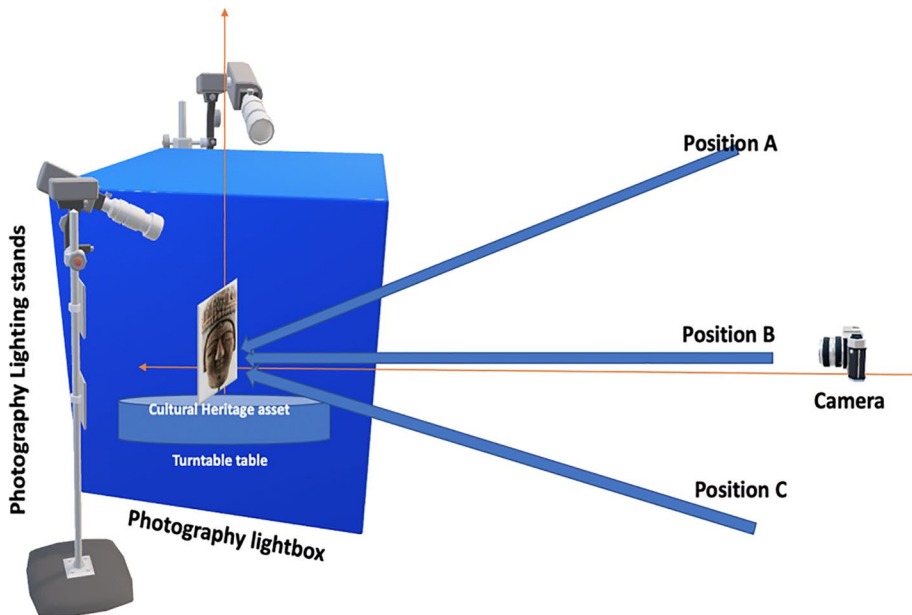
Fig. 8 Camera position setup
