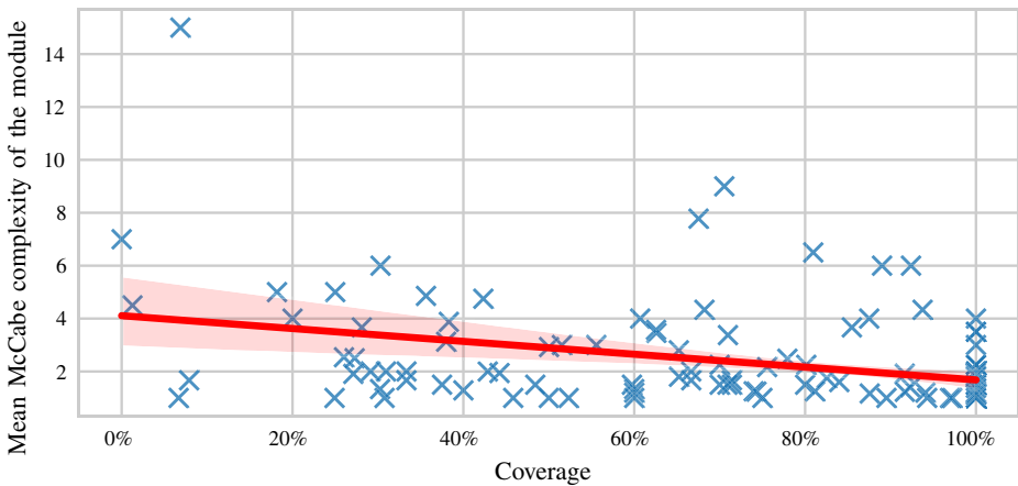
Fig. 6 Mean coverage for DynaMOSA with type information correlated to the mean McCabe cyclomatic complexity of a module's functions; the red line shows the linear regression fitted to the data (Pearson r = -0.365 , p = 3.00 \times 10^{-5} )
