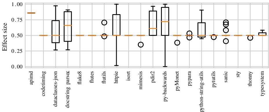
Fig. 7 Effect-size distributions per project for DynaMOSA. \hat{A}_{12} > 0.500 indicates that DynaMOSA-TypeHints performed better than DynaMOSA-NoTypeHints; vice versa for \hat{A}_{12} < 0.500
