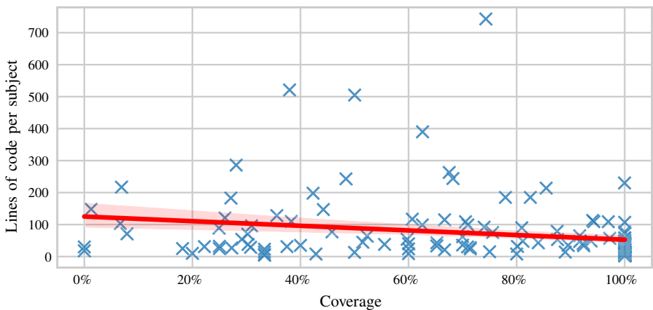
Fig. 5 Mean coverage for DynaMOSA with type information correlated to the lines of code per module; the red line shows the linear regression fitted to the data (Pearson r = -0.211 , p = 0.0143 )
