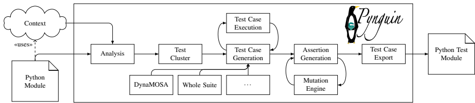
Fig. 1 The different components of PYNGUIN (taken from Lukaszcyk and Fraser (2022))
