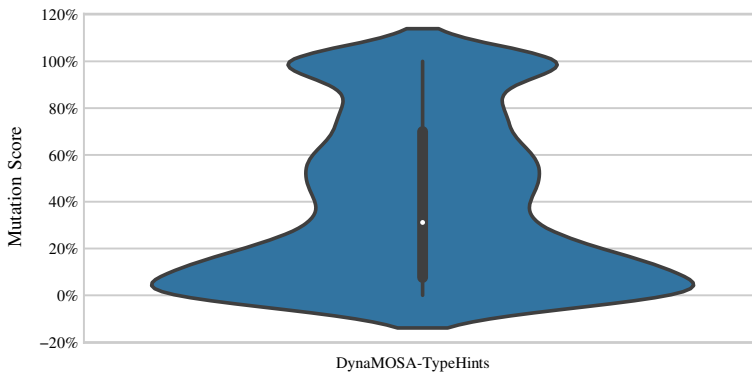
Fig. 8 A violinplot showing the distribution of the mutation scores for the used DynaMOSA configuration in our experiment for RQ3
