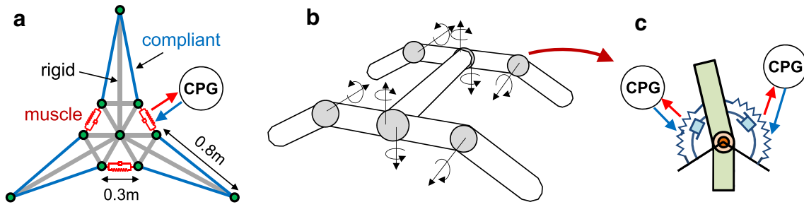
Fig. 10 Simulated robots. (a) 3-arm 2D mass-spring-damper swimmer. (b) 8 DoF quadruped. (c) Antagonistic torsional muscles for a joint of quadruped
