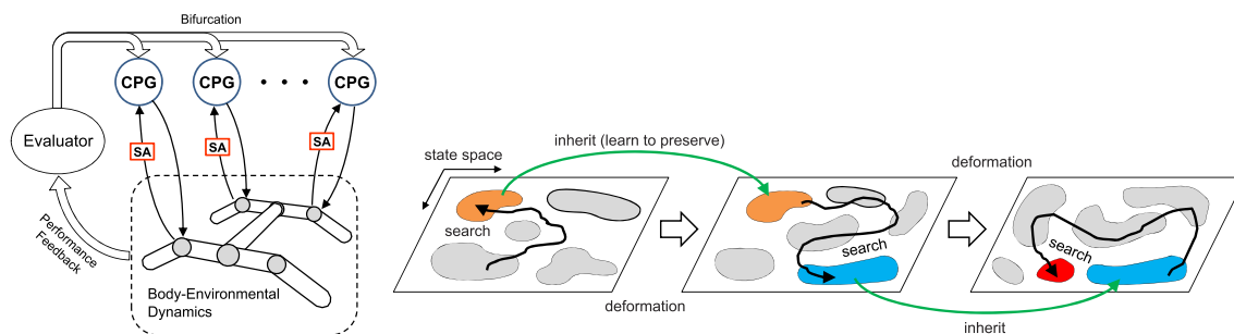
Fig. 8 The overall chaotic exploration concept for motor behaviours. Left: Performance feedback is transformed into a descending input to all CPGs which acts as a bifurcation parameter. The level of chaotification of the system is inversely proportional to its performance. Actuator sensory signals pass through a homeostatic adaptive process (SA). Right: Overall search dynamics of the method. Chaotic exploration samples the population of attractors
