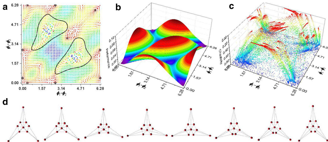
Fig. 11 Chaotic exploration of 2D swimmer. a behavioural stability landscape. 6 stable points (on a 2-torus surface) and 2 periodic transitions emerged symmetrically due to the radial symmetry of the robot morphology. b Performance landscape. 3 stable points have the highest performances (i.e. locomotion speed), whereas the other 3 points
