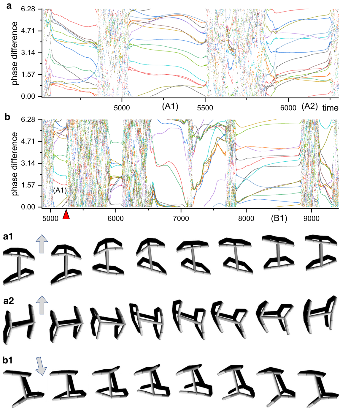
Fig. 12 Chaotic exploration of Quadruped. a An example of the time courses of phase differences between CPG-1 and the other 15 CPGs during exploration. Two high performing locomotor behaviours are shown as (a1; quadruped walking gait) and (a2; side-walk like gait) with corresponding snapshots. b A scenario for the realtime recovery
