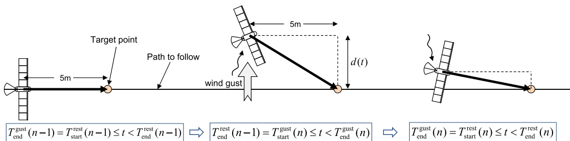
Fig. 16 Flapping wing flyer evaluation strategy
