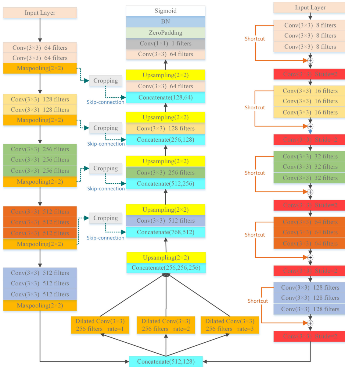
Fig. 4 DCU-Net model structure for image splicing forgery detection. There are two encoders on the left and right sides. The input is tampered image and residual image. At the bottom is the feature fusion module, the first is the fusion of image features and residual
