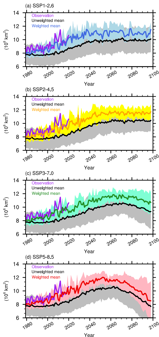
Fig. 5. Time series of wintertime newly formed sea-ice extent in the unweighted and weighted CMIP6 multimodel ensemble under the (a) SSP1-2.6, (b) SSP2-4.5, (c) SSP3-7.0, and (d) SSP5-8.5 scenarios. The colored curves and bands indicate the weighted multimodel mean and spread, respectively. The black curves and gray bands indicate the unweighted multimodel mean and spread, respectively. The purple solid curves represent observations.
