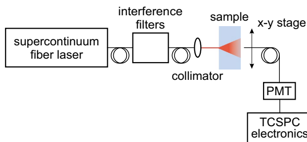
Fig. 3 Schematic diagram of the setup used for the TOF experiments. PMT photomultiplier, TCSPC time-correlated single-photon counting
