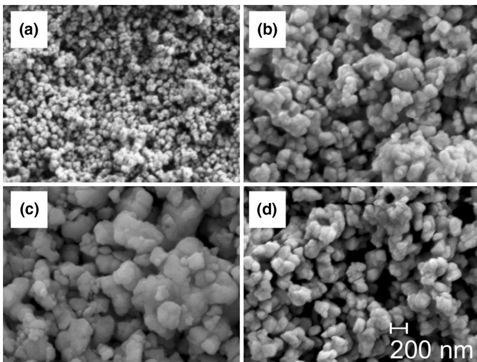
Fig. 1 Scanning electron microscope images of selected nanoporous material: a type Z1, b type Z5, c type Z9, and d sample of the type Z7
